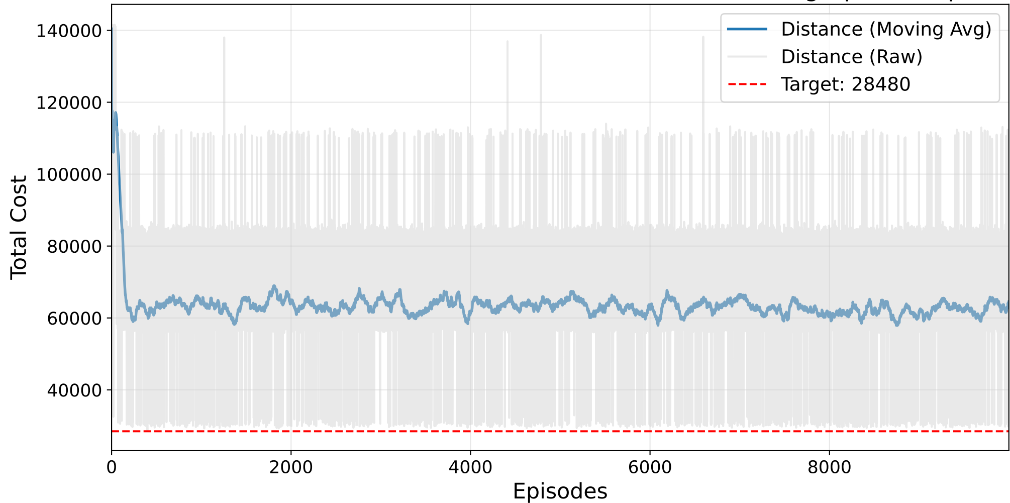
Final GAUSSIAN PROCESS Masked AutoRL-SOP Training - p43.2.sop
